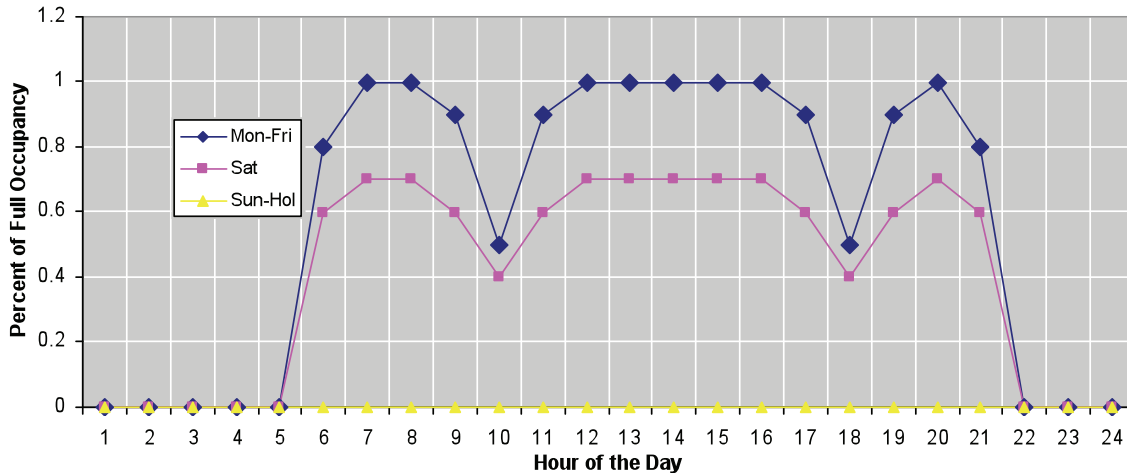
Figure 3 Occupancy Schedules
