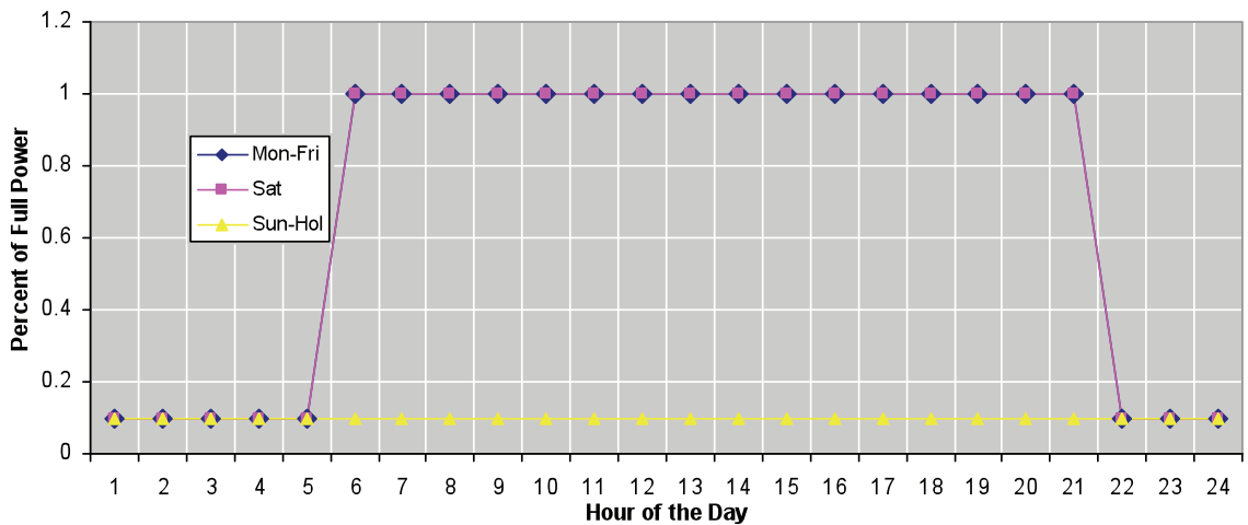
Figure 6 Lighting Schedules
