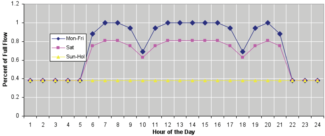
Figure 5 Infiltration Schedules
